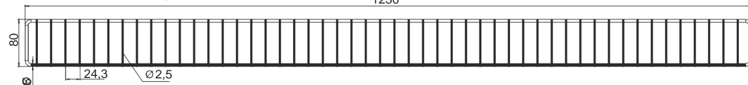
Front stop for shelving 1230x80 mm V2 1230
