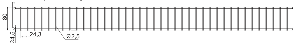
Front stop for shelving 1230x80 mm 1230
