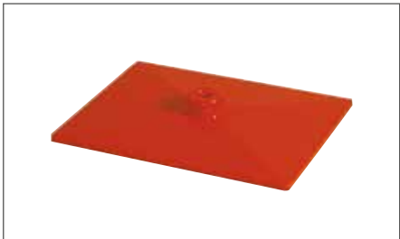
BASE K Made of plastics, with centred tube holder to take tubes Ø 12 mm, in OEK standard colors. Size: 200 x 150 mm. Also available with zincd metal inlay. base K | 20350-xx with metal inlay | 20351-xx
