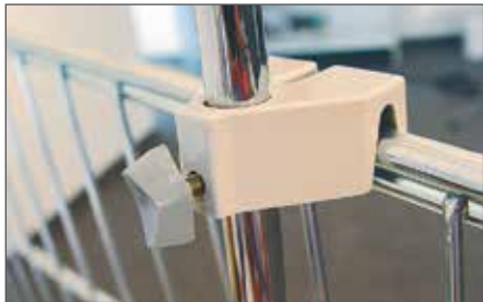
SHOWCARD HOLDER DK DK wire holder (pair) made of grey plastic, suits wires with Ø 4 - 8 mm, with a vertical wire distance of min. 18 mm, chromium tube adjustable 320 - 620 mm, frame A4 and T-piece in OEK standard colors. 35424-xx
