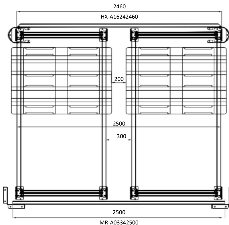
Example of using corner and front guard with fender beams
