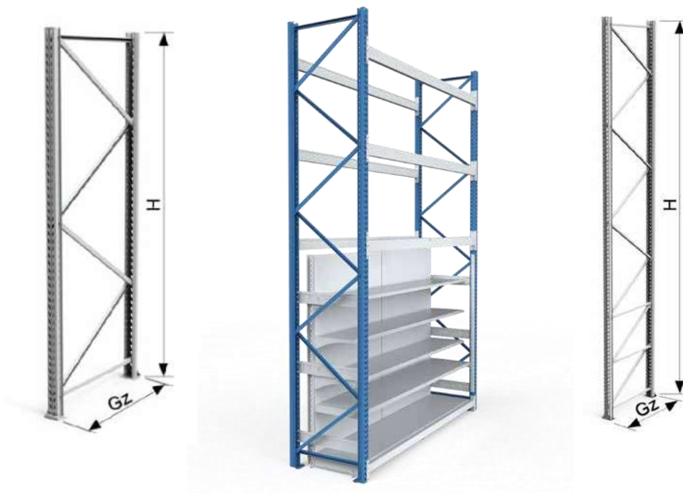
FRAME 82 0185 (S) DOUBLE INTEGRATION 2 FRAMES
