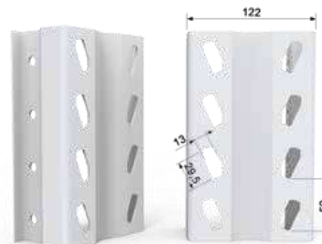
HX122 PILLAR PROFILE
