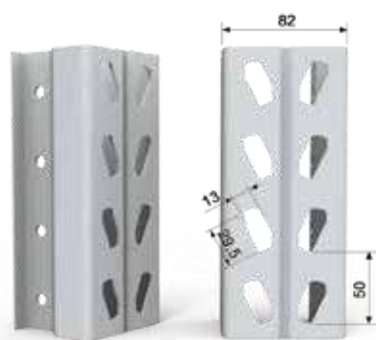
HX82 PILLAR PROFILE
